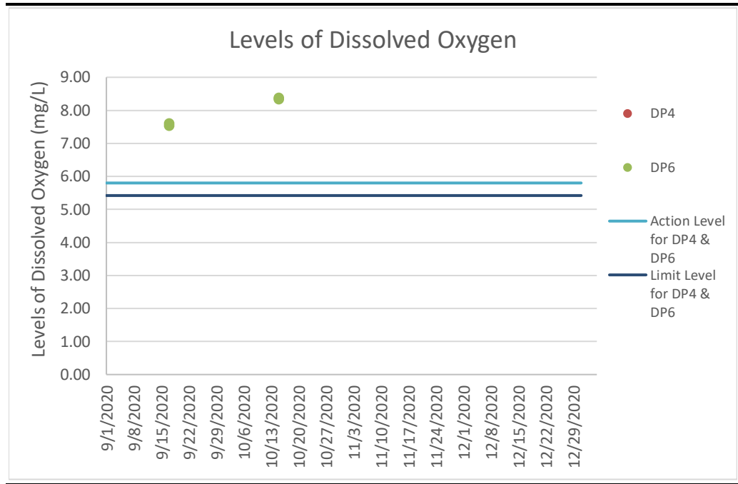
Figure F1.1 Graphical Presentation for Surface Water Quality Monitoring (DO)
